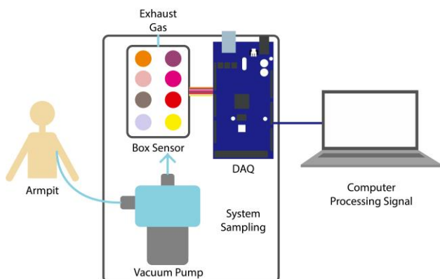
Figure. 2 E-nose architecture
