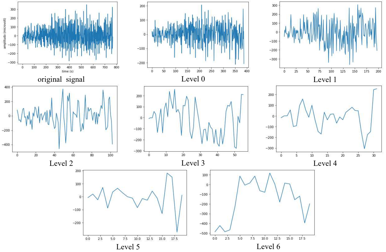
Figure 3. DWT decomposition for EEG Signal using Biorthogonal 2.4
