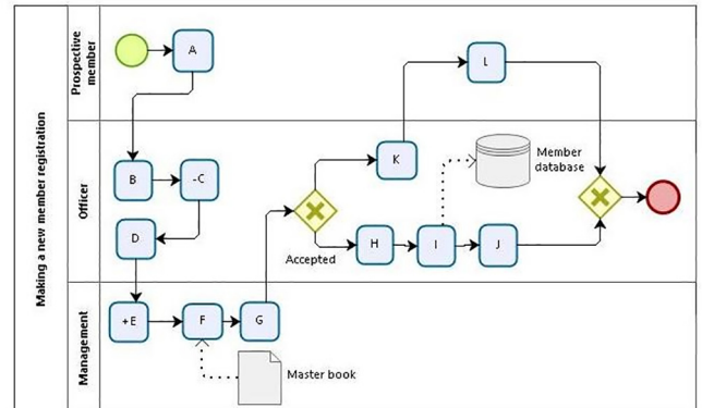
Fig. 4. The BPMN diagram generated for case study 9.
