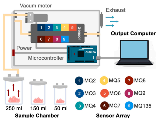
Fig. 2. E-Nose system design with MQ family sensors.
