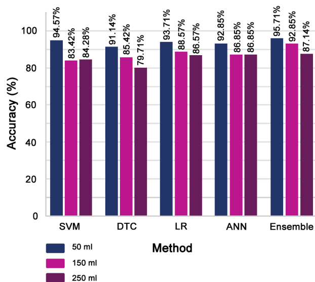
Fig. 9. Accuracy comparison chart between sample chamber and classifier method.
