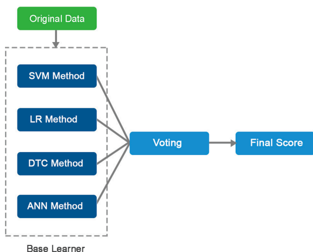
Fig. 5. Ensemble method with voting approach.
